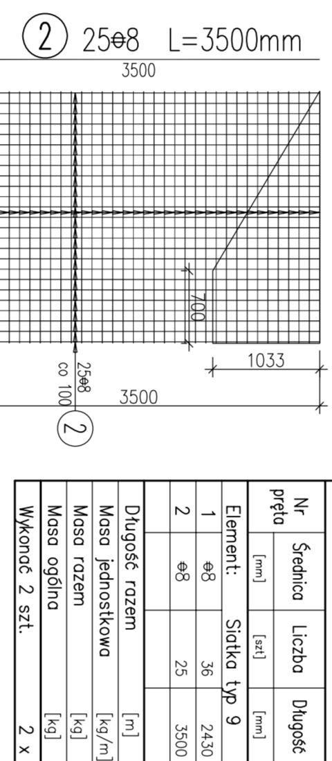
Siatka "Typ 9" ø8 100x100mm
