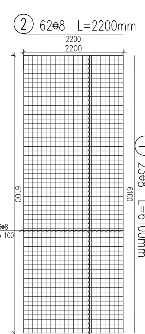
Siatka "Typ 5" ø8 100x100mm
