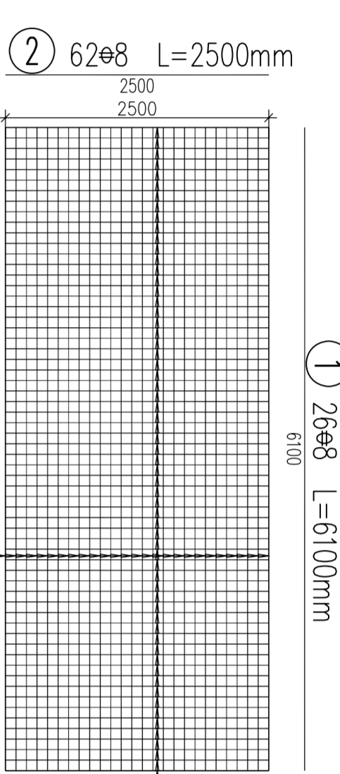
Siatka "Typ 6" ø6 100x100mm
