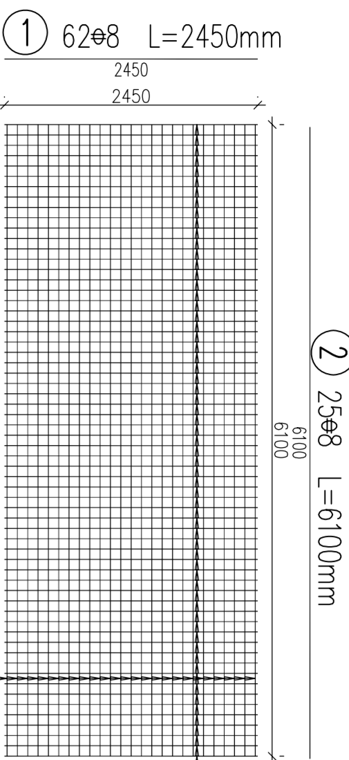
Siatka "Typ 1" ø8 100x100mm
