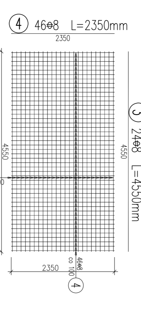
Siatka "Typ 3d" ø8 100x100mm
