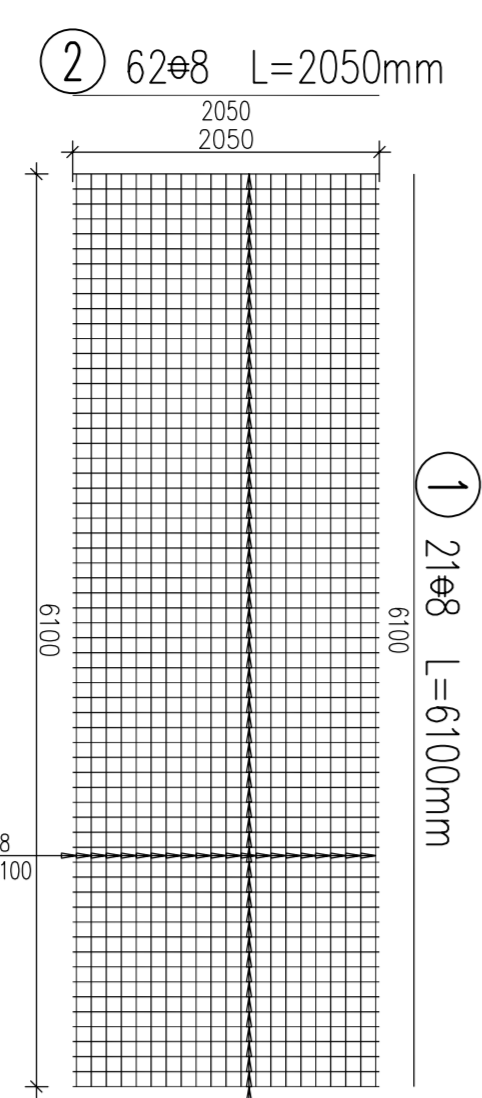
Siatka "Typ 4" ø8 100x100mm
