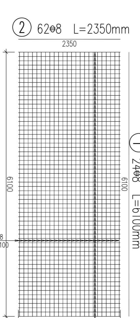
Siatka "Typ 3" ø8 100x100mm
