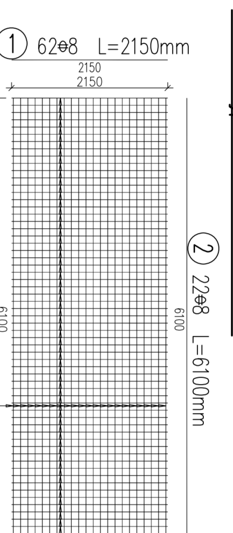
Siatka "Typ 7" ø8 100x100mm
