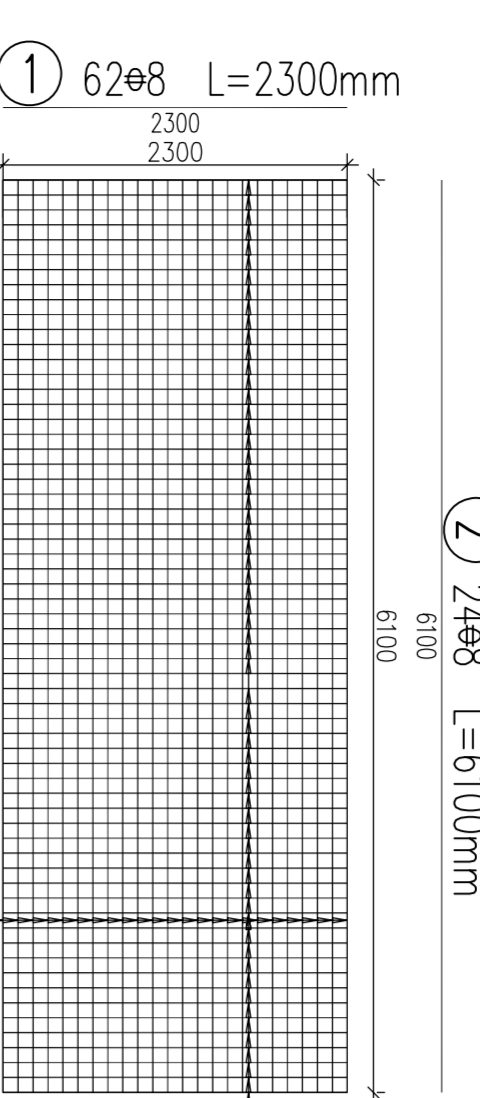
Siatka "Typ 2" ø8 100x100mm
